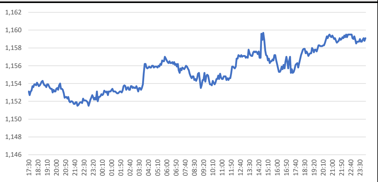
€/ $ Spot
