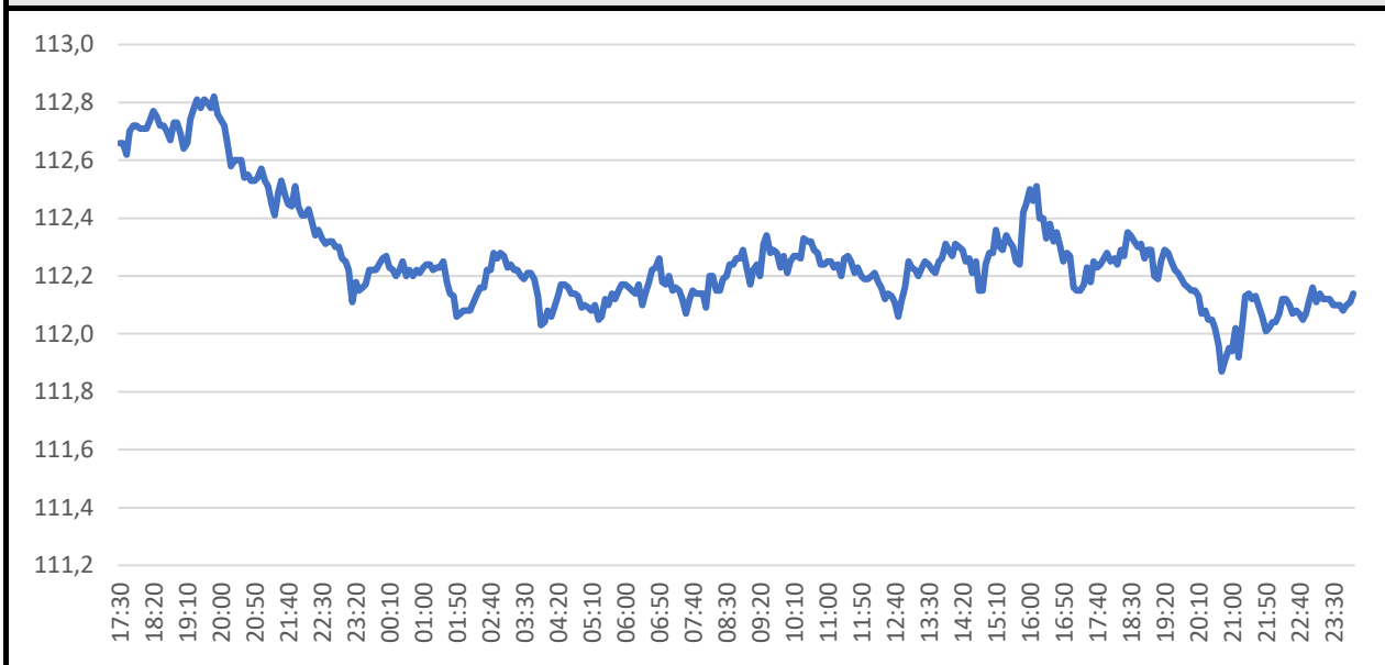
$/Y Spot
