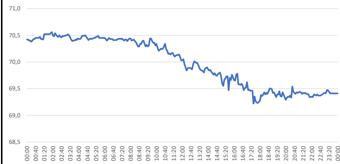
BRENT Future
